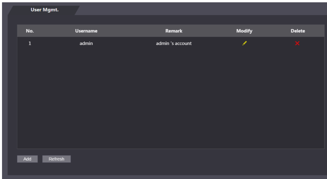
Figure 4-27 User management
