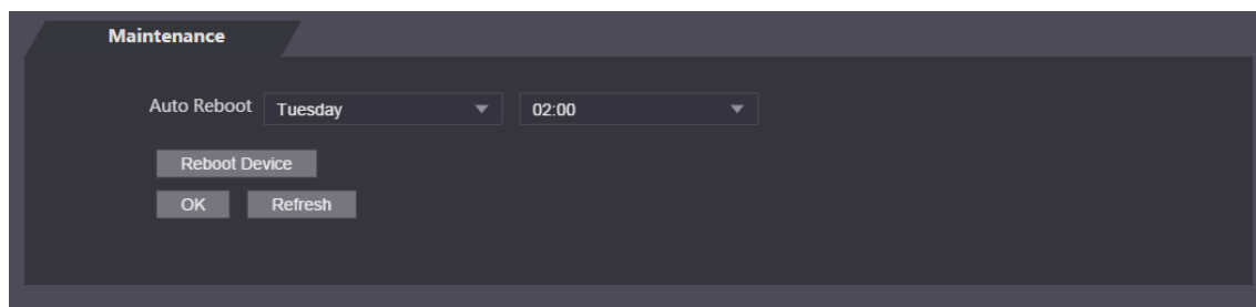
Figure 4-28 Maintenance
