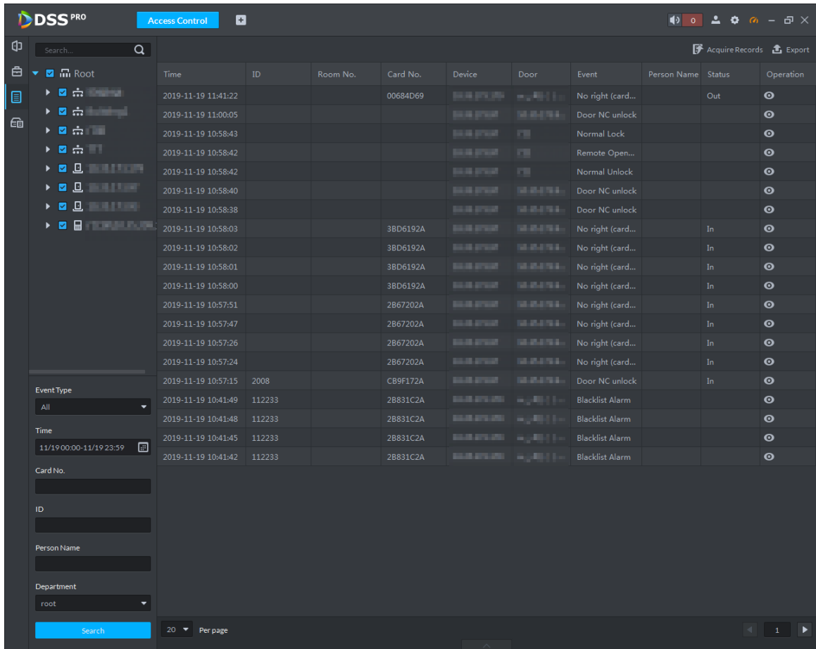
Figure 6-28 Log search
